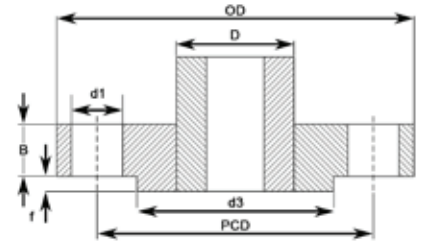
20 mm Nominal Bore (3/4") - Pipe OD 26.67mm
