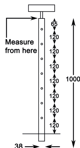
7 Hole Upright Post
